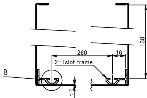
Sectional view A-A Scale 1 : 2
