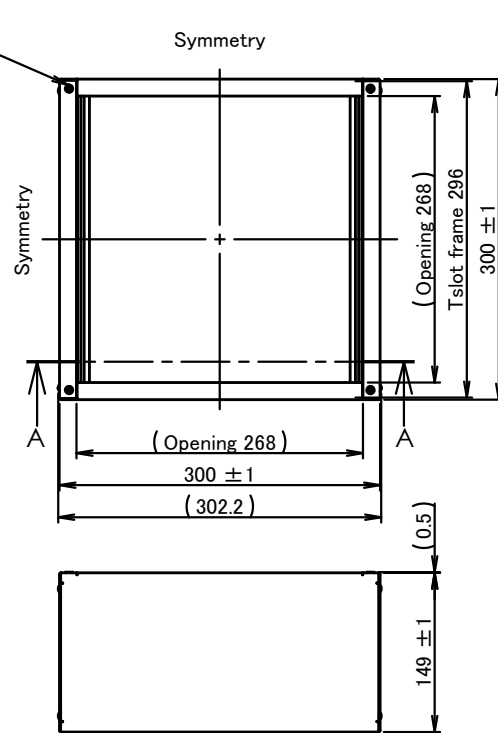
Sectional view A-A Scale 1 : 2
