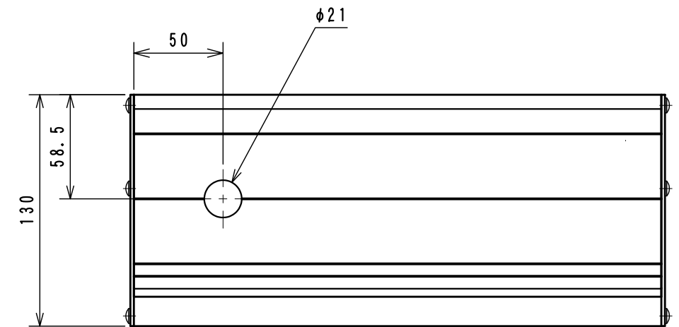
Arrow View A
