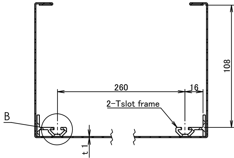
Sectional view A-A Scale 1 : 2
