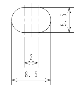
Detail C Scale 2:1 2 Places
