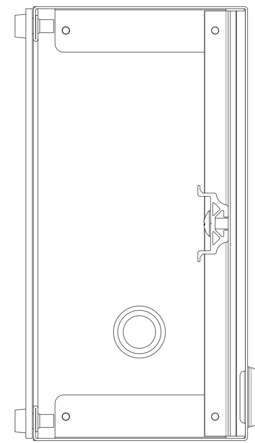
Sectional view B-B
